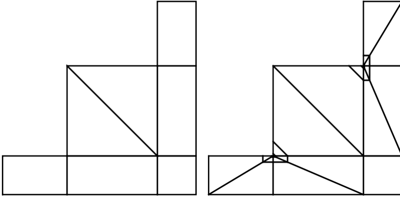
Figure 6: Meshing setup for cross in square
