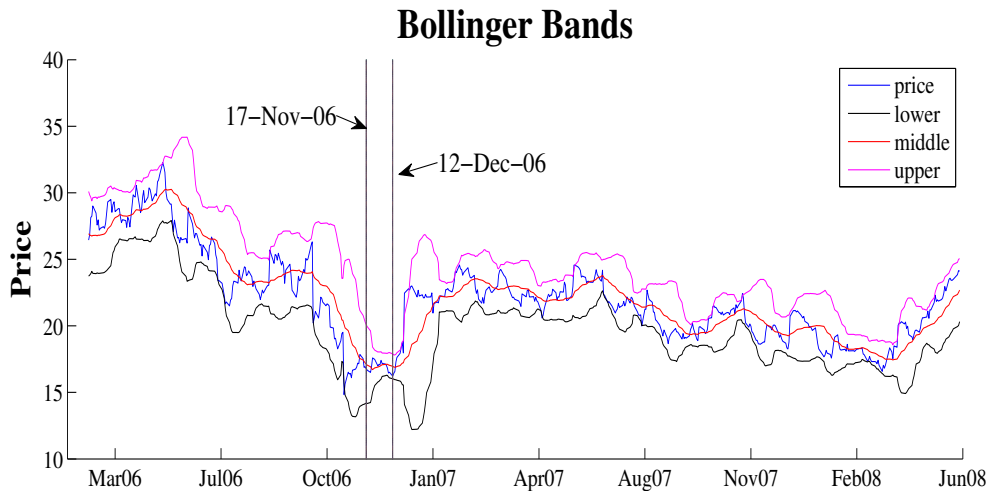
Figure 1: Bollinger bands along with the adjusted closing prices of Red Hat stock.
