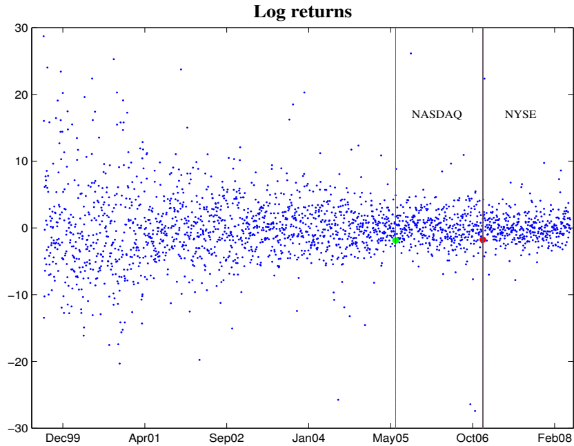
Figure 3: Sample sets are constructed from the most recent historical log returns with 368 units each one. The vertical lines shows the regions where each set belongs.
