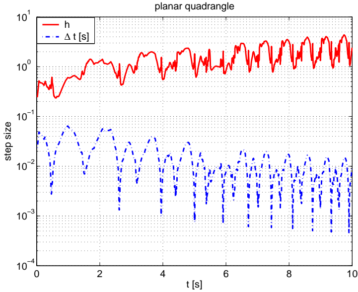
Figure 6.7: Step sizes of the planar quadrangle.
