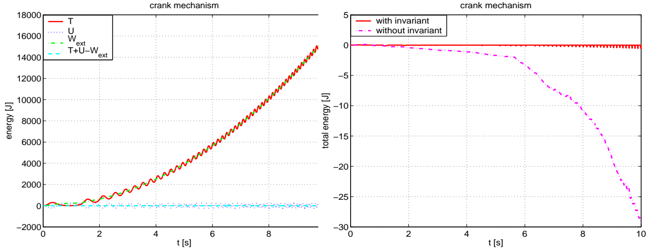
Figure 6.8: On the left: energies of the crank mechanism when the conservation of the energy is imposed. On the right: the total energy with and without conservation of energy.
