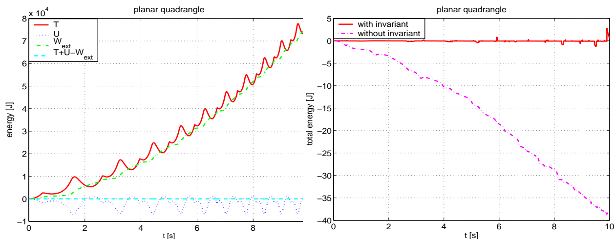
Figure 6.6: On the left: energies of the planar quadrangle when the conservation of the energy is imposed. On the right: the total energy with and without conservation of energy.
