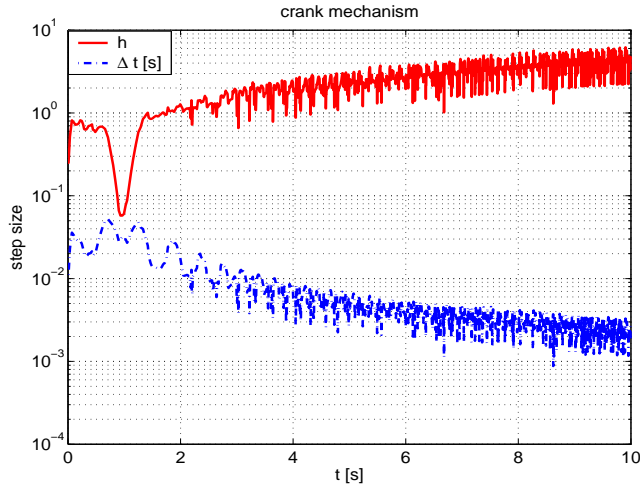
Figure 6.9: Step sizes of the crank mechanism.
