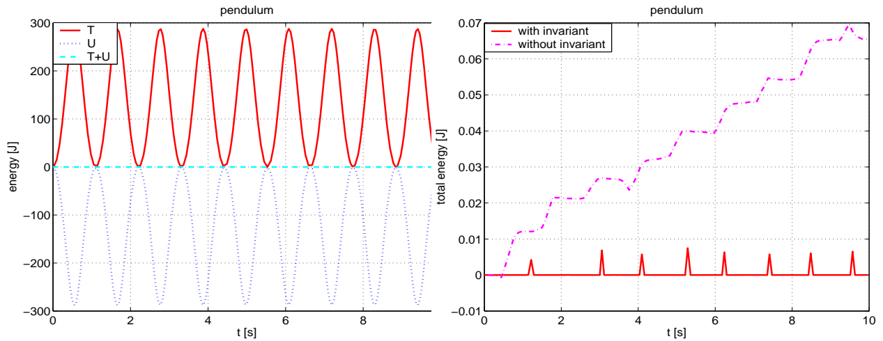
Figure 6.4: On the left: energies of the pendulum when the conservation of the energy is imposed. On the right: the total energy with and without conservation of energy.
