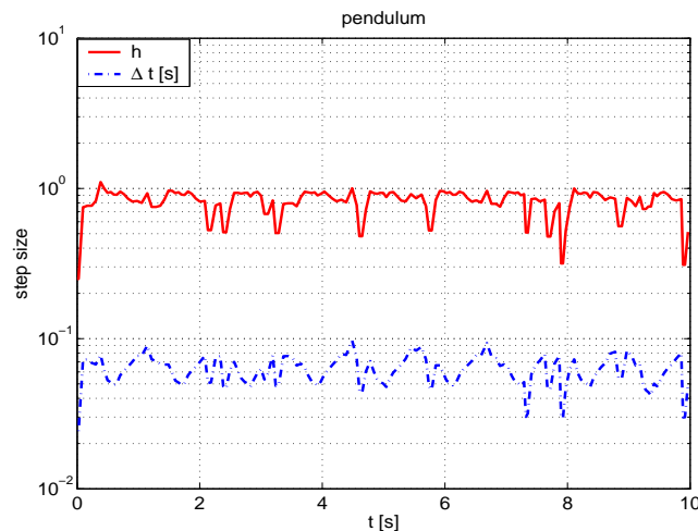
Figure 6.5: Step sizes of the pendulum.
